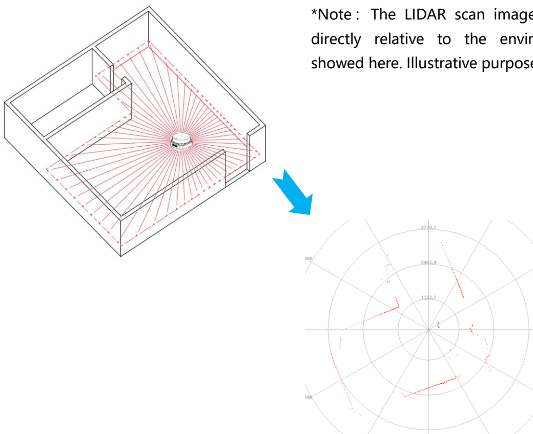
Figure 1-3 The Obtained Environment Map from RPLIDAR S2 Scanning
